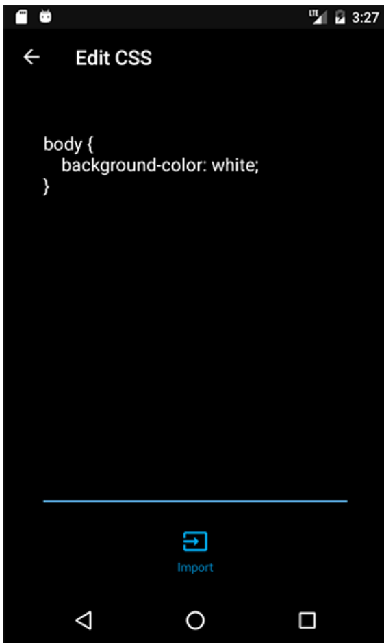
Figure 16. CSS Editor
