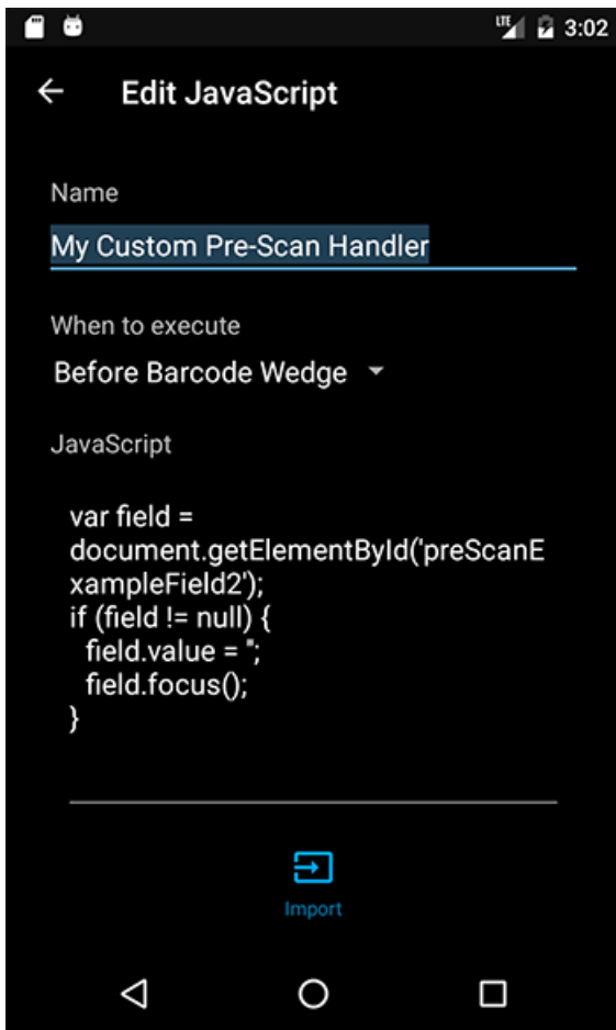
Figure 15. JavaScript Editor
