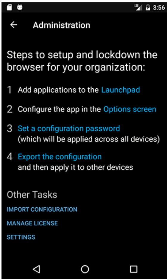
Figure 11. Administration Screen
