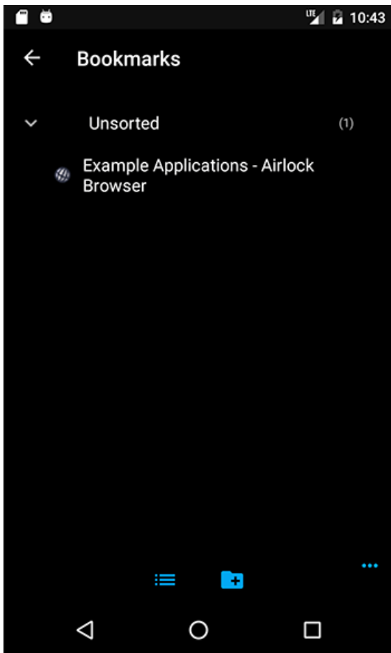
Figure 18. Bookmarks screen
