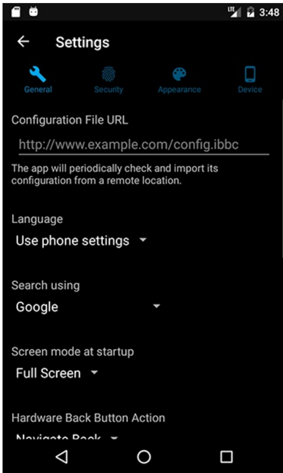
Figure 3. Settings Screen
