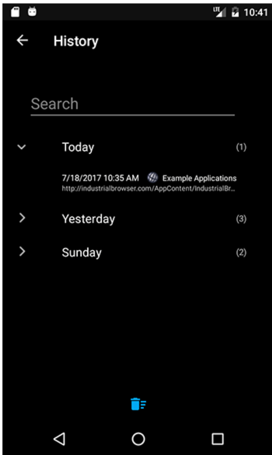
Figure 17. History screen
