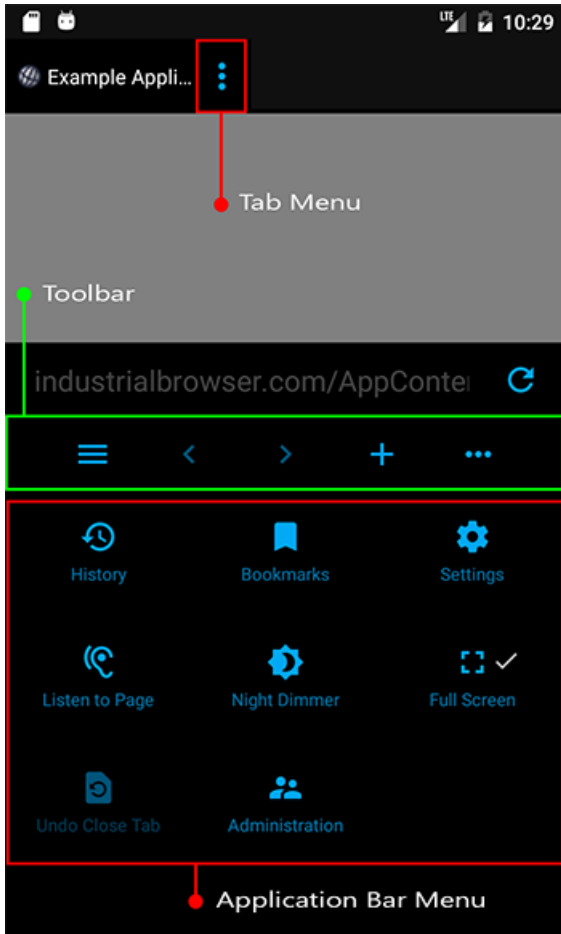
Figure 6. Application bar menu, toolbar, and tab menu
