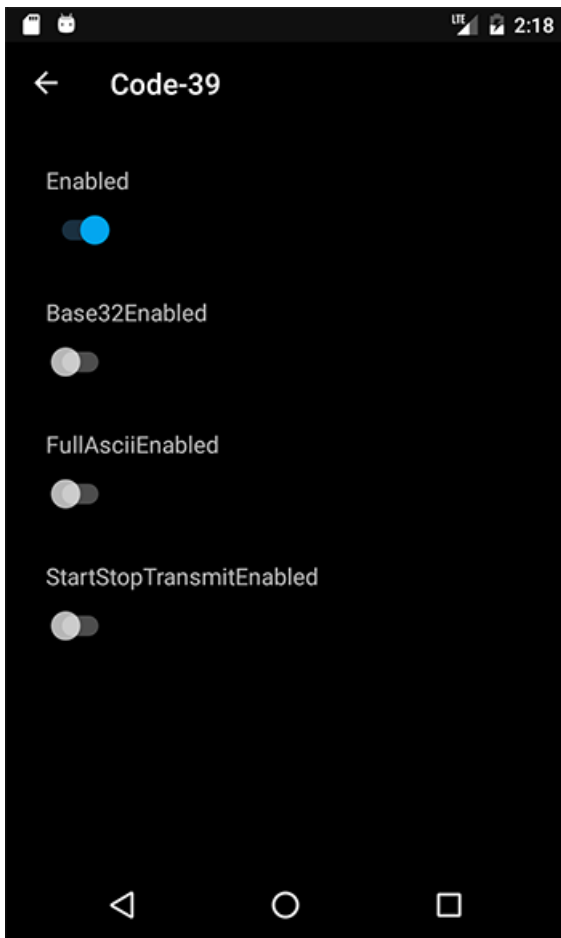
Figure 10. Symbology screen
